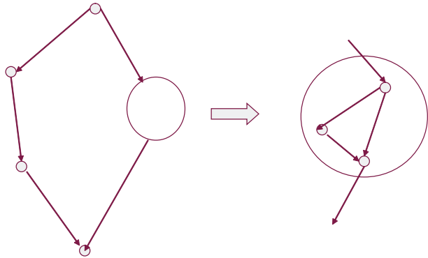
Fig. 5. Subgraph
