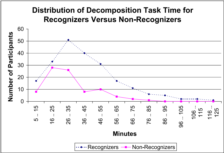
Fig. 6. Distribution of time taken to complete design decomposition task, separated into recognizers and non-recognizers
