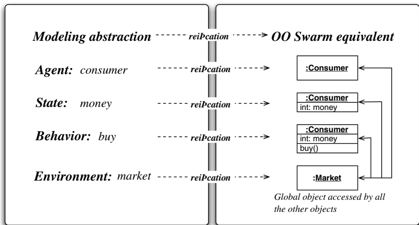
Fig. 1. Modeling abstraction reified into OO equivalent
